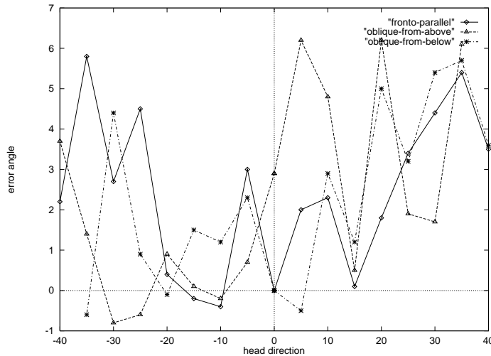
Figure 4: The difference between the ground-truth and recovered pose angles as a function of the ground-truth angle.
