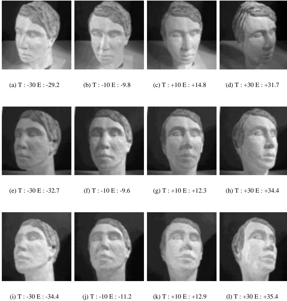
Figure 3: A series of views of a plaster bust in which the camera direction is approximately fronto-parallel, oblique from above and oblique from below. The ground-truth angles are denoted by “T” and the estimated angles by “E”.
