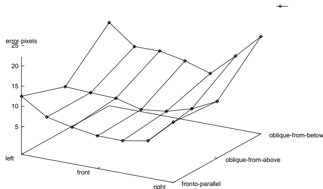
Figure 2: The positional accuracy of automatically segmented points.
