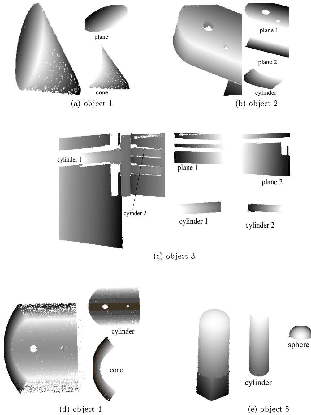
Figure 1: Examples of the objects used in the experiments with the extracted surfaces.
