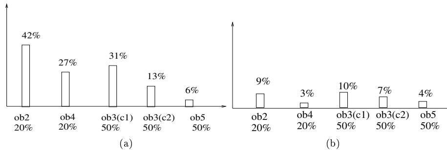
Figure 2: shape bias in the cylinder estimates (ob:object, c1:cylinder1,etc.). (a) with the AD technique, (b) with the AED technique
