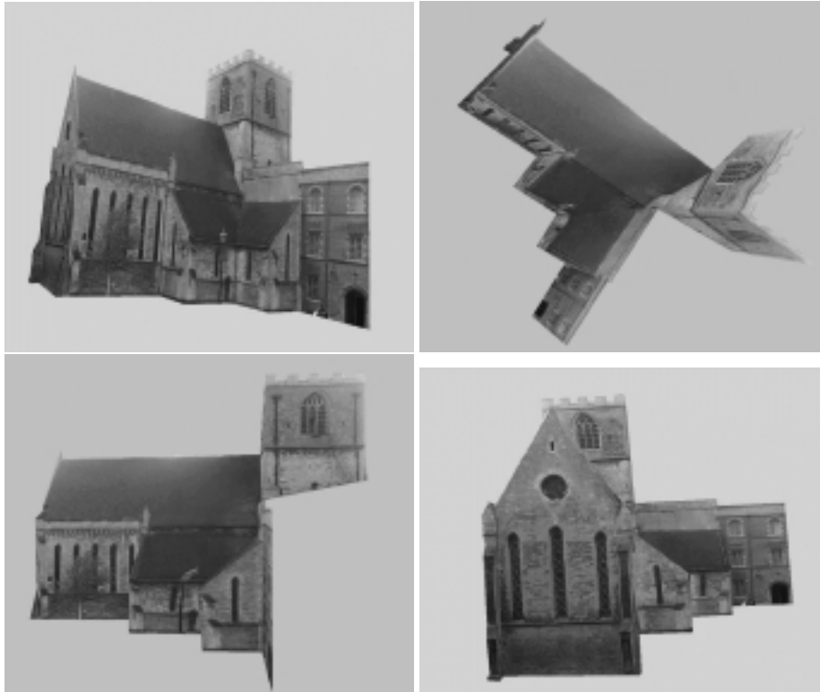
Figure 4: The 3D model can be output in VRML format and viewed from new viewpoints. Four novel views are shown of the reconstructed model. The texture is automatically extracted from the pair of original uncalibrated photographs.
